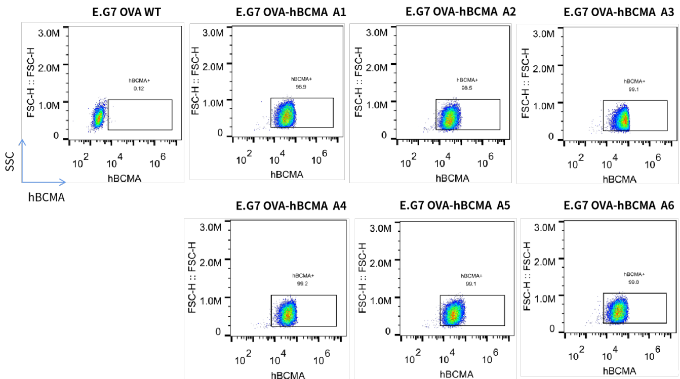
Fig1. hBCMA expression on in vitro cultured cells of E.G7 OVA-hBCMA
