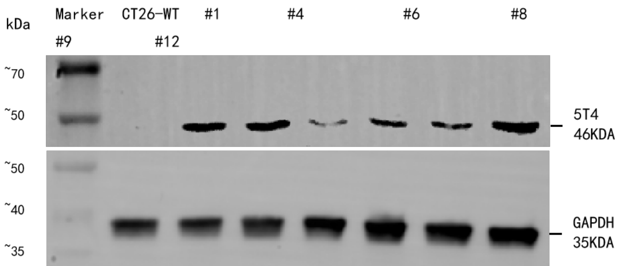
Fig1. h5T4 expression on in vitro cultured cells of CT26-h5T4
