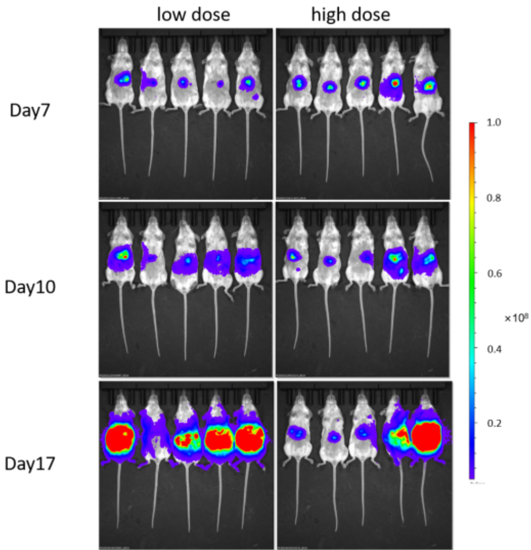
Fig5. Bioluminescence imaging of H22-Luc allogeneic mouse model
