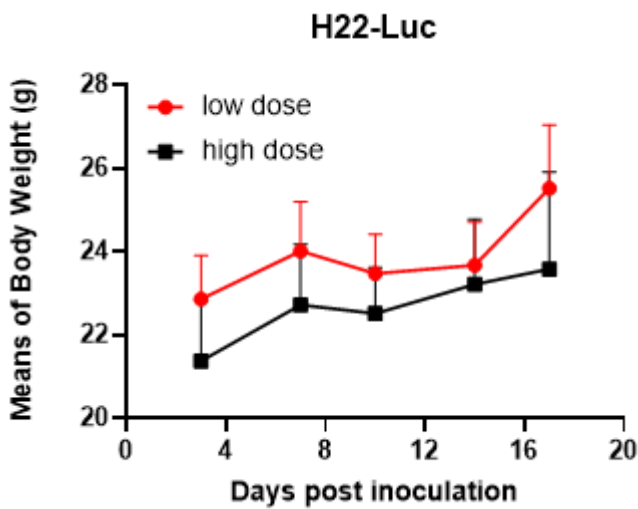
Fig3. Body weight change of H22-Luc allogeneic mouse model (n=5)
