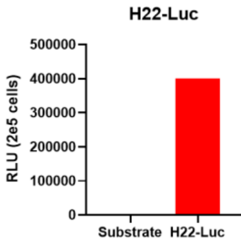
Fig1. Luciferase activity assay of H22-Luc cell line
