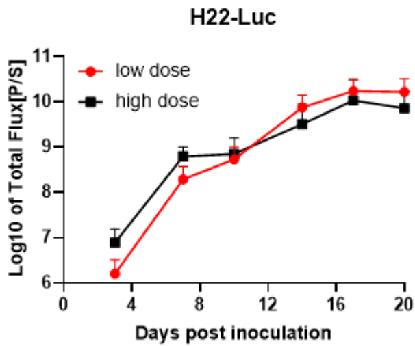
Fig2. Signal increase curve in H22-Luc allogeneic mouse (n=5)
