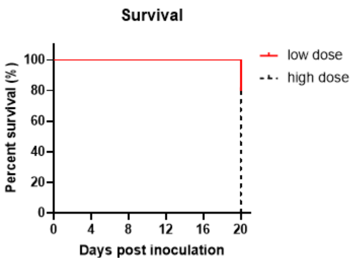
Fig4. Survival curve in H22-Luc allogeneic mouse model (n=5)
