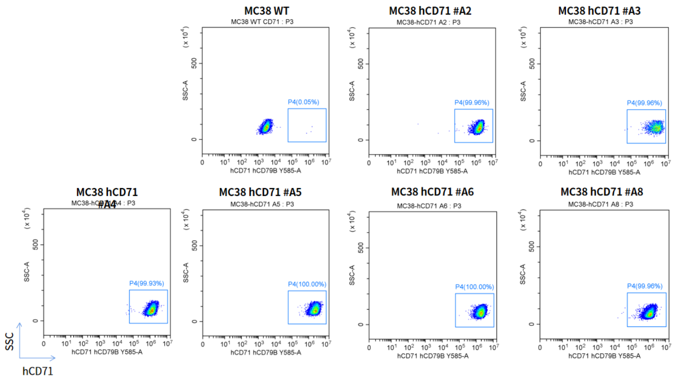
Fig1.hCD71 expression on in vitro cultured cells of MC38-hCD71-Tg
