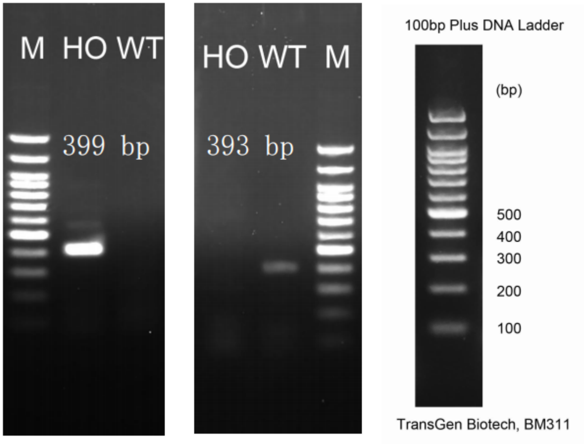
Fig1. Detection of hMELTF mRNA in hMELTF knockin mice.
