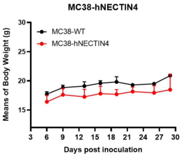
Figure 3. Body weight change of MC38-hNECTIN4 syngeneic model (n=4).
