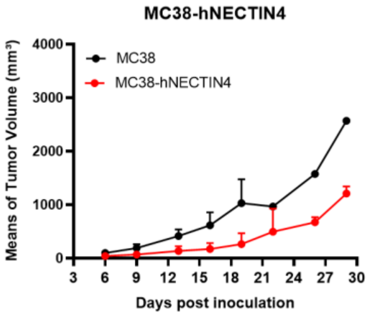
Figure 2. Tumor growth curve of MC38-hNECTIN4 syngeneic model (n=4).
