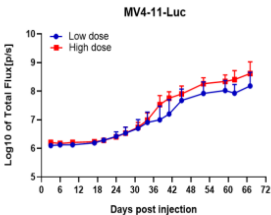
Figure 1. Luciferase activity assay of MV4-11-Luc cell line
