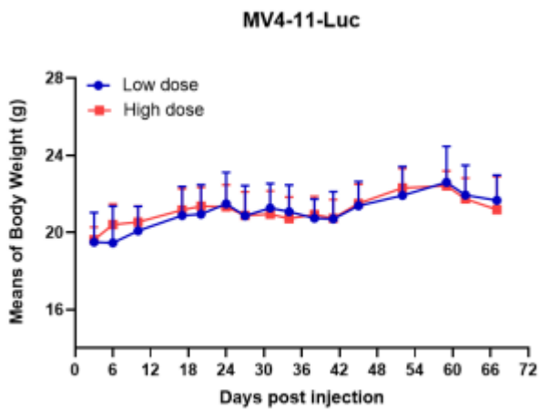
Figure 2. Signal increase curve in MV4-11-Luc xenograft model (n=5)
