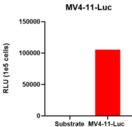
Figure 1. Luciferase activity assay of MV4-11-Luc cell line
