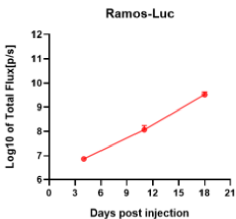
Figure 2. Signal increase curve in Ramos-Luc xenograft model (n=5)
