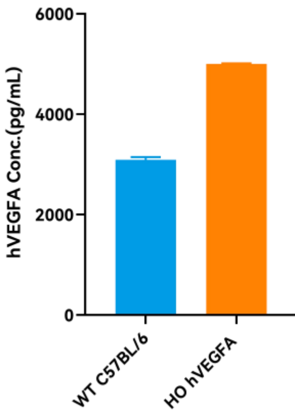
Fig 2. Detection of hVEGFA expression in lung homogenate by ELISA.
