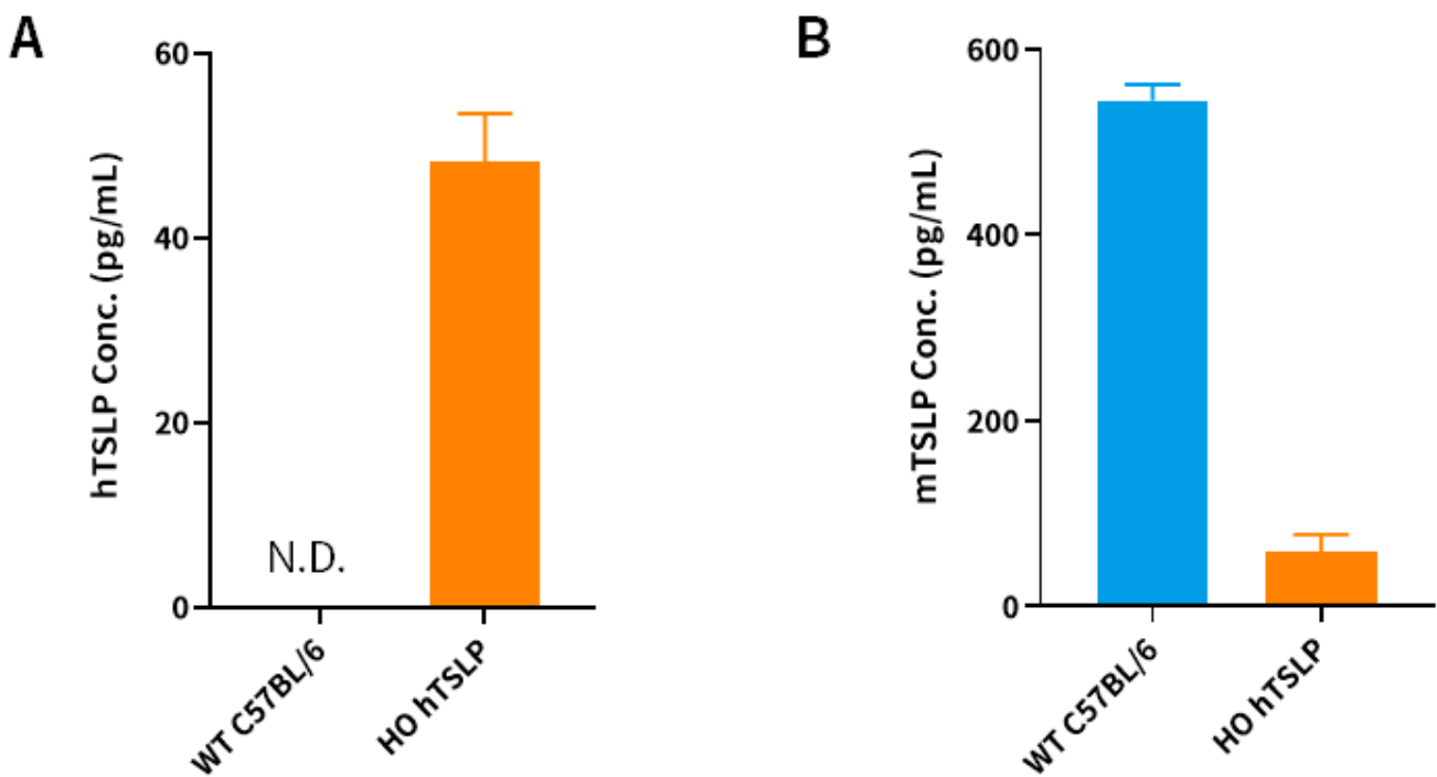
Fig.2 Detection of hTSLP and mTSLP expression in thymus homogenate by ELISA (n=5).
